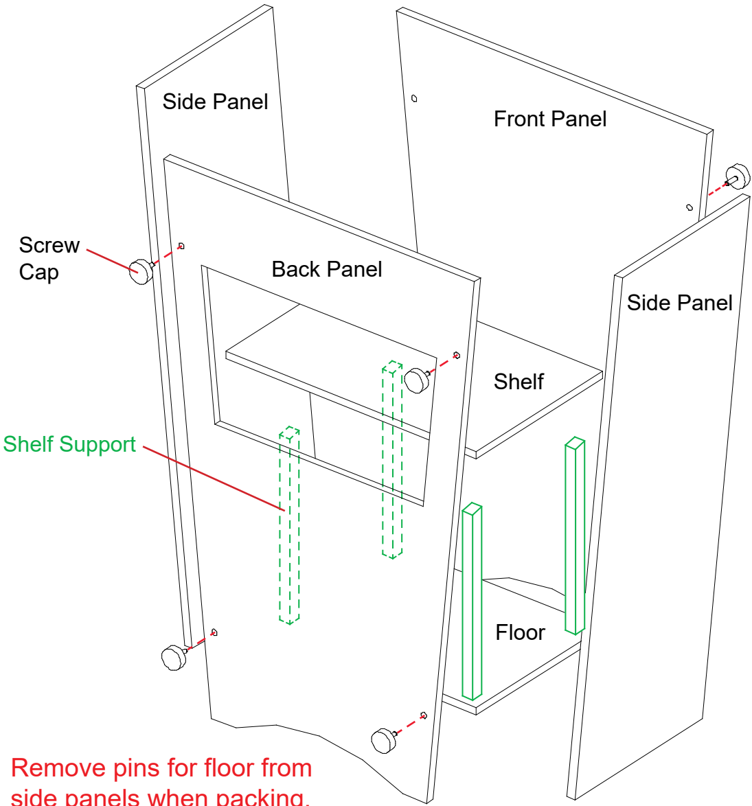
Pedestal Base Assembly BACK VIEW
